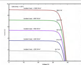
Current-Voltage Characteristic
